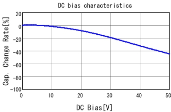
GCM21BR71H224KA37 C-DC bias capchange, 25.0degC, AC1.
