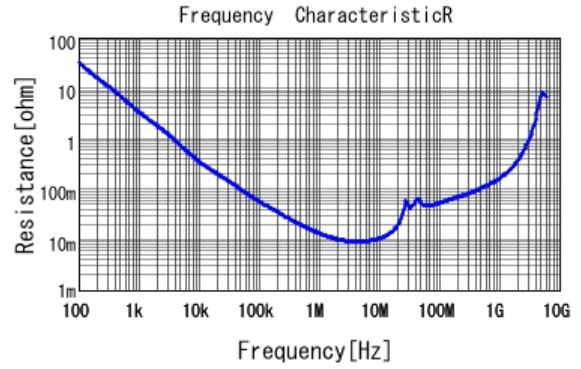
GCM21BR71H224KA37 R DC0V, 25degC
