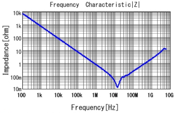
GCM21BR71H224KA37 |Z| DC0V, 25degC
