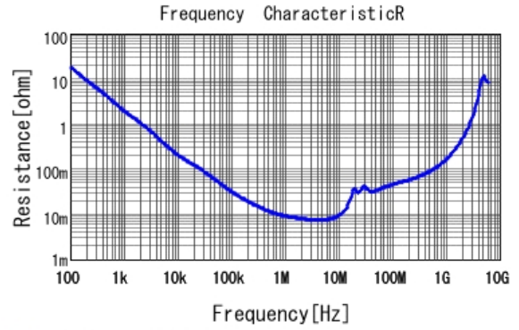
■ GCM21BR71H474KA55 R DC0V, 25degC
