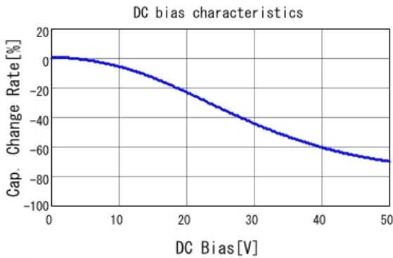
■ GCM21BR71H474KA55 C-DC bias capchange, 25.0degC, AC1.
