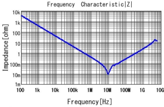
■ GCM21BR71H474KA55 |Z| DC0V, 25degC
