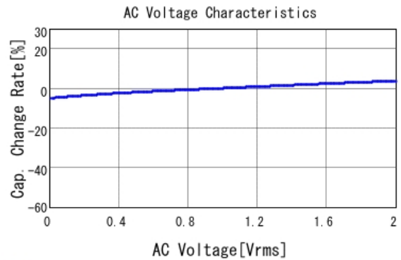
■ GCM21BR71H474KA55 C-AC Voltage capchange, DC0V, 25.0d
