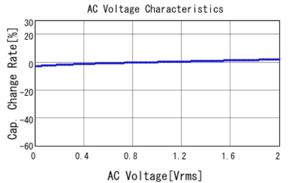
GCM21BR72A473KA37 C-AC Voltage capchange, DCOV, 25.0d
