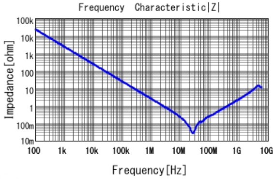
GCM21BR72A683KA37 |Z| DCOV, 25degC
