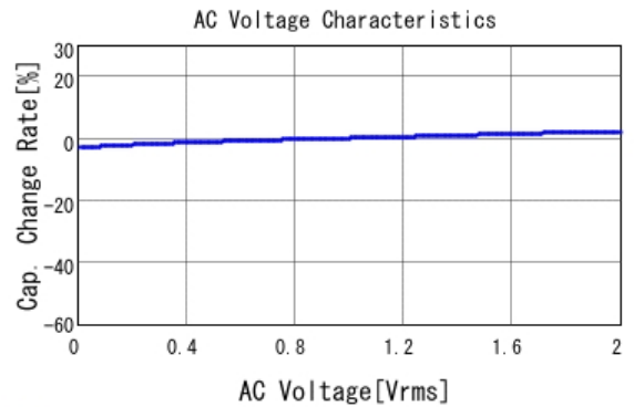
GCM21BR72A683KA37 C-AC Voltage capchange, DCOV, 25.0d
