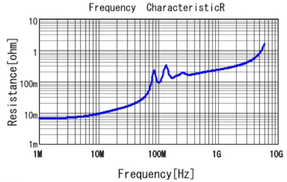
■ GCM3195C1H223JA16 R DCOV, 25degC
