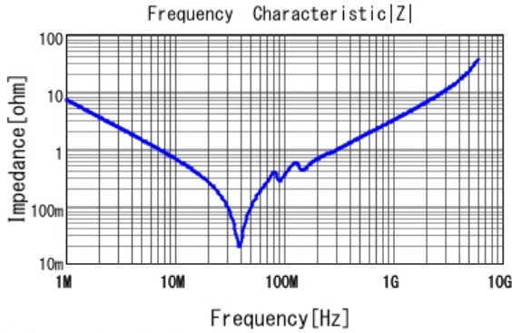
■ GCM3195C1H223JA16 |Z| DCOV, 25degC
