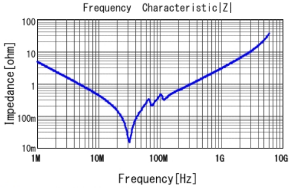
■ GCM3195C1H333JA16 |Z| DCOV, 25degC
