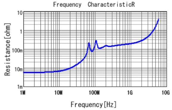
■ GCM3195C1H333JA16 R DCOV, 25degC
