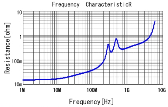
■ GCM3195C2A272JA16 R DCOV, 25degC
