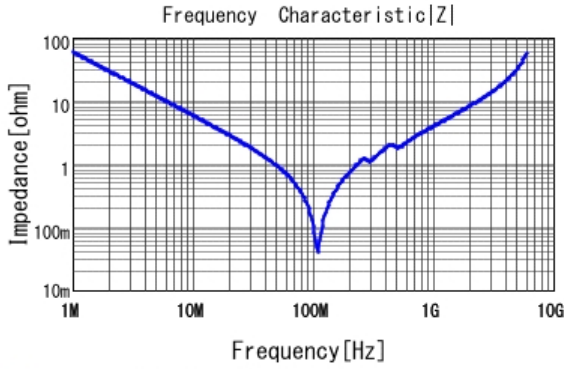
■ GCM3195C2A272JA16 |Z| DCOV, 25degC
