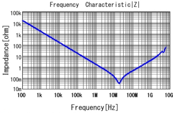
GCM319R72A104KA37 |Z| DC0V, 25degC
