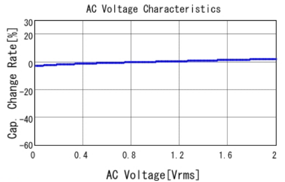
GCM319R72A104KA37 C-AC Voltage capchange, DC0V, 25.0d
