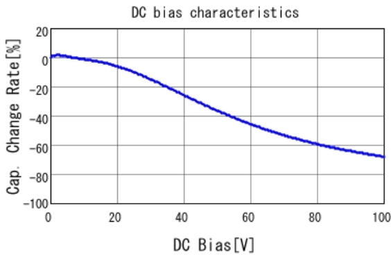
GCM319R72A104KA37 C-DC bias capchange, 25.0degC, AC1.
