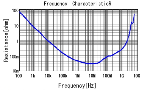
GCM319R72A104KA37 R DC0V, 25degC
