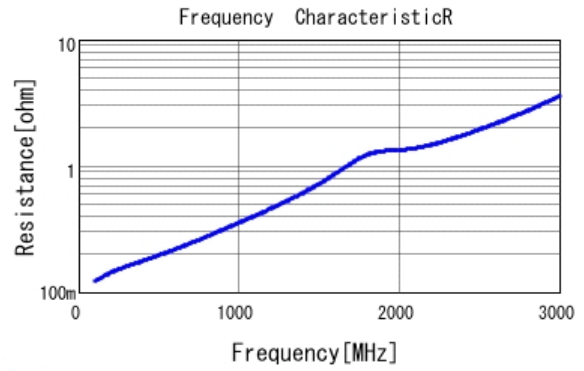
■ GCM31A5C2J151JX01 R DC0V, 25degC
