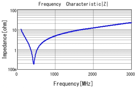
■ GCM31A5C2J151JX01 |Z| DC0V, 25degC
