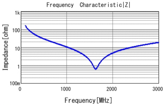
■ GCM31A5C3A100JX01 |Z| DC0V, 25degC
