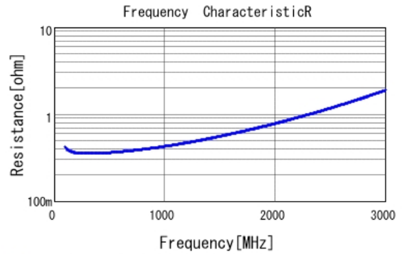
■ GCM31A5C3A100JX01 R DC0V, 25degC
