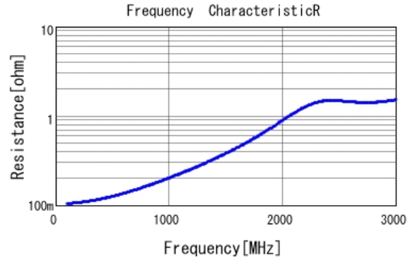
■ GCM31A5C3A101JX01 R DC0V, 25degC
