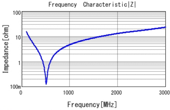
■ GCM31A5C3A101JX01 |Z| DC0V, 25degC
