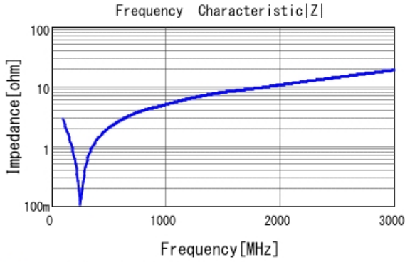
■ GCM31A7U2J471JX01 |Z| DC0V, 25degC
