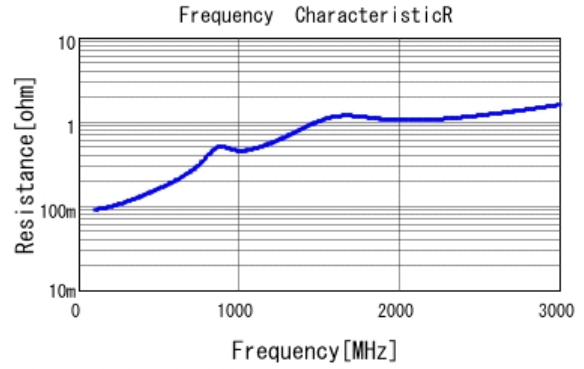
■ GCM31A7U2J471JX01 R DC0V, 25degC
