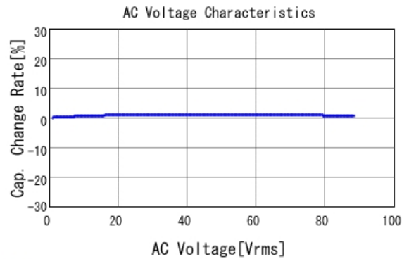
■ GCM31B7U2E103JX01 C-AC Voltage capchange, DC0V, 25.0d
