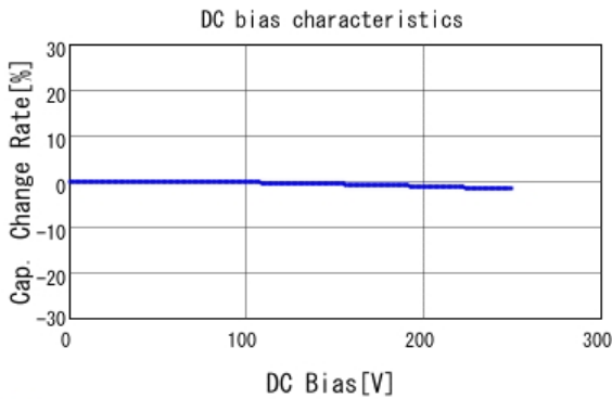
■ GCM31B7U2E103JX01 C-DC bias capchange, 25.0degC, AC1V
