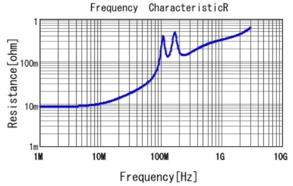
■ GCM31B7U2E103JX01 R DC0V, 25degC
