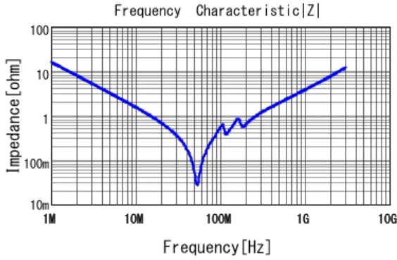
■ GCM31B7U2E103JX01 |Z| DC0V, 25degC
