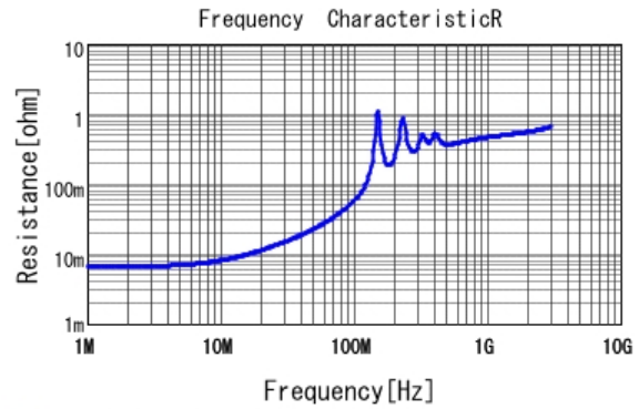
■ GCM31C7U2J472JX03 R DC0V, 25degC
