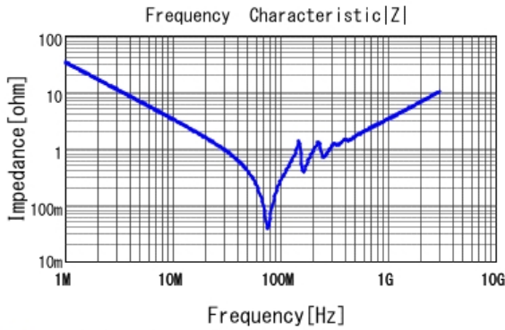
■ GCM31C7U2J472JX03 |Z| DC0V, 25degC
