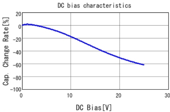
■ GCM31CC71E106KA03 C-DC bias capchange, 25.0degC, AC1.
