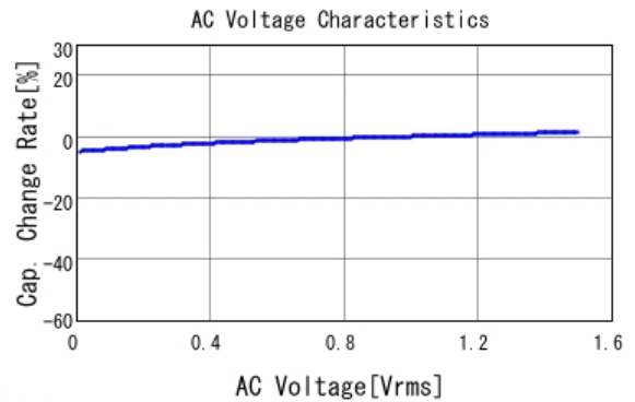
■ GCM31CC71E106KA03 C-AC Voltage capchange, DCOV, 25.0d
