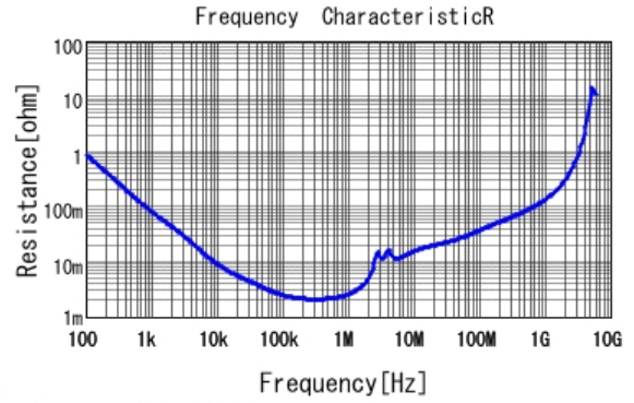
■ GCM31CC71E106KA03 R DCOV, 25degC
