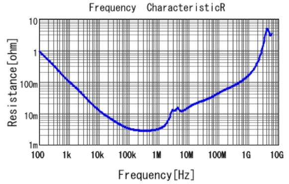
GCM31CR71A106KA64 R DCOV, 25degC
