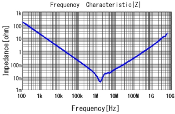
GCM31CR71A106KA64 |Z| DCOV, 25degC
