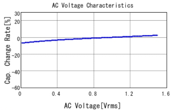
GCM31CR71A106KA64 C-AC Voltage capchange, DCOV, 25.0d
