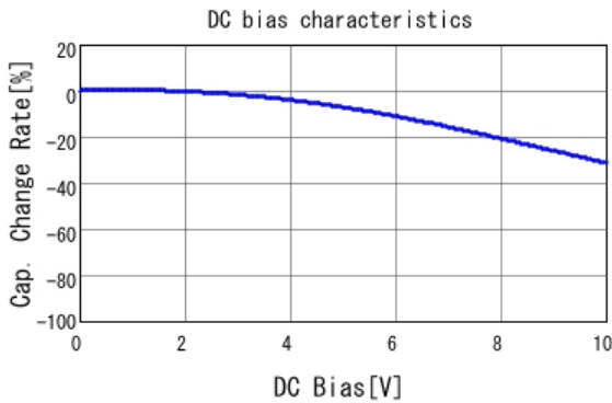
GCM31CR71A106KA64 C-DC bias capchange, 25.0degC, AC1.
