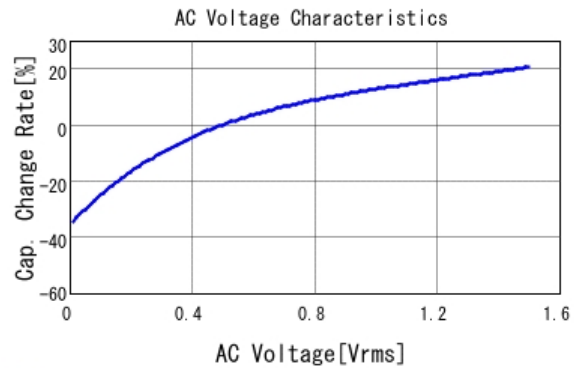
GCM31CR71A226KE02 C-AC Voltage capchange, DCOV, 25.0d
