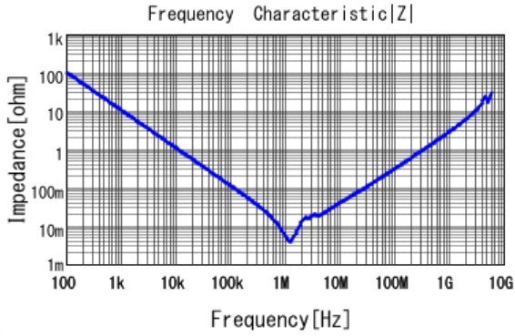
GCM31CR71A226KE02 |Z| DCOV, 25degC
