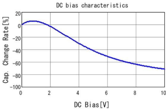
GCM31CR71A226KE02 C-DC bias capchange, 25.0degC, AC0.
