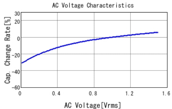
■ GCM31CR71C106KA64 C-AC Voltage capchange, DCOV, 25.0d
