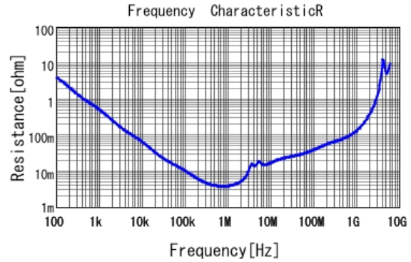
■ GCM31CR71C106KA64 R DCOV, 25degC
