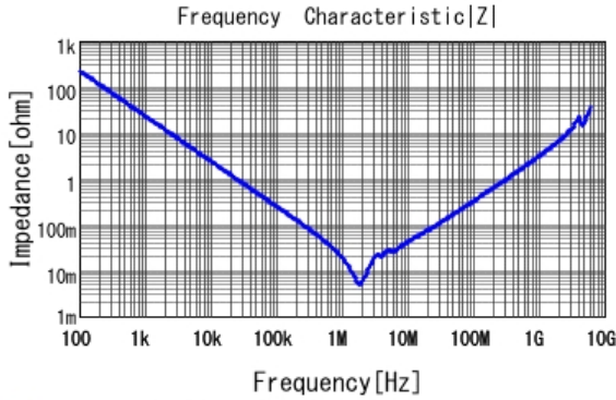
■ GCM31CR71C106KA64 |Z| DCOV, 25degC
