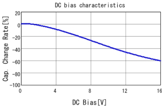
■ GCM31CR71C106KA64 C-DC bias capchange, 25.0degC, AC1.
