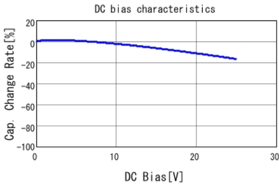
■ GCM31CR91E105KA37 C-DC bias capchange, 25.0degC, AC1.
