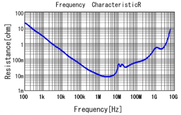
■ GCM31CR91E105KA37 R DCOV, 25degC
