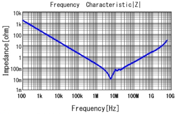
■ GCM31CR91E105KA37 |Z| DCOV, 25degC
