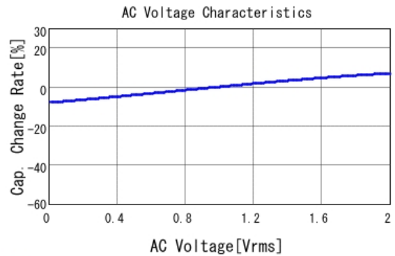
■ GCM31CR91E105KA37 C-AC Voltage capchange, DCOV, 25.0d
