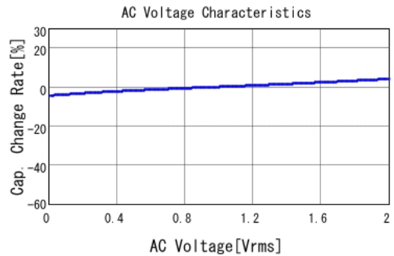
■ GCM31MR71E105KA37 C-AC Voltage capchange, DCOV, 25.0d
