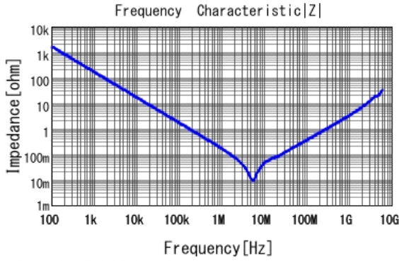
■ GCM31MR71E105KA37 |Z| DCOV, 25degC
