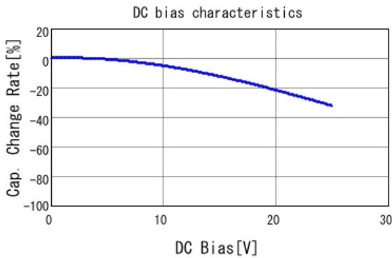
■ GCM31MR71E105KA37 C-DC bias capchange, 25.0degC, AC1.
