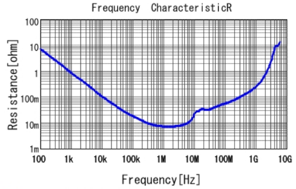
■ GCM31MR71E105KA37 R DCOV, 25degC
