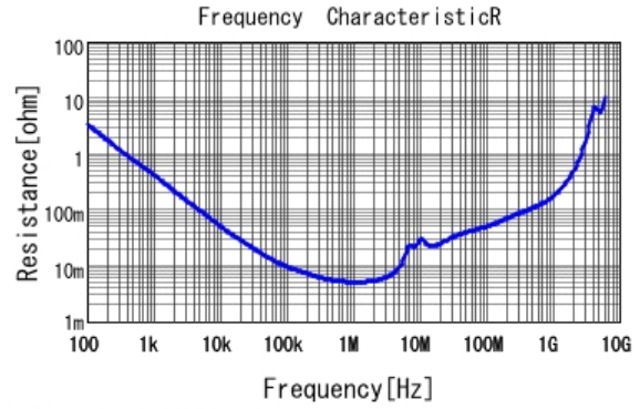
■ GCM31MR71E225KA57 R DCOV, 25degC
