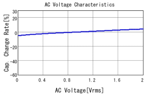
■ GCM31MR71E225KA57 C-AC Voltage capchange, DCOV, 25.0d
