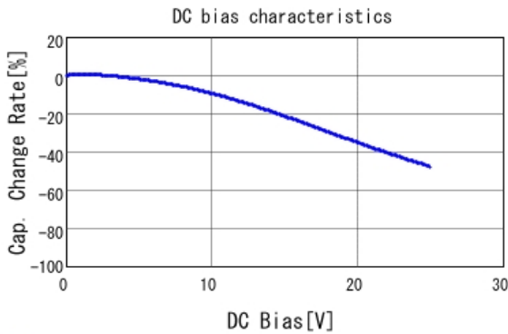
■ GCM31MR71E225KA57 C-DC bias capchange, 25.0degC, AC1.
