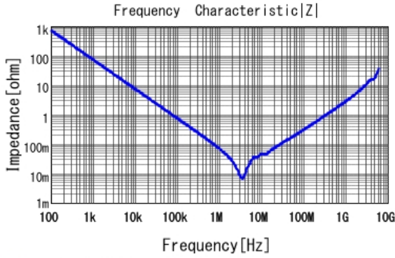
■ GCM31MR71E225KA57 |Z| DCOV, 25degC
