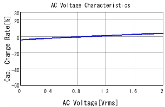
GCM31MR71H105KA55 C-AC Voltage capchange, DCOV, 25.0d
