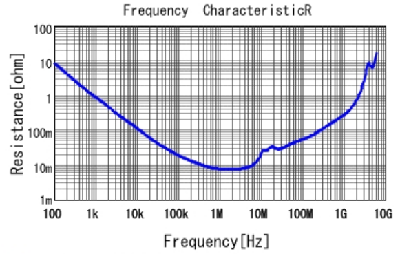
GCM31MR71H105KA55 R DCOV, 25degC
