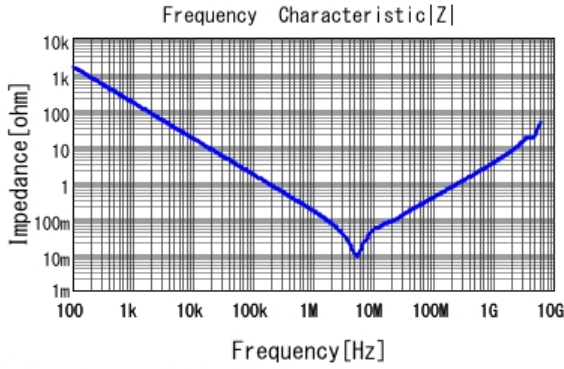
GCM31MR71H105KA55 |Z| DCOV, 25degC
