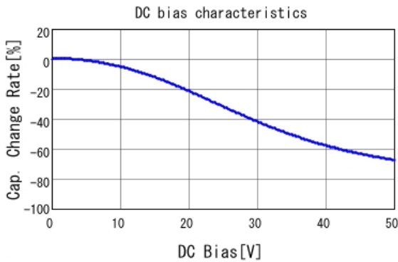
GCM31MR71H105KA55 C-DC bias capchange, 25.0degC, AC1.
