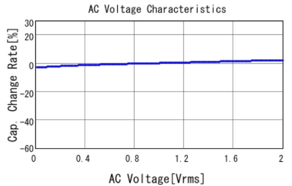
GCM31MR72A224KA37 C-AC Voltage capchange, DC0V, 25.0d
