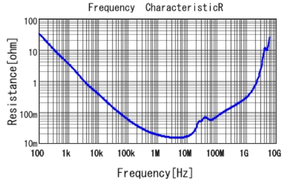
GCM31MR72A224KA37 R DC0V, 25degC
