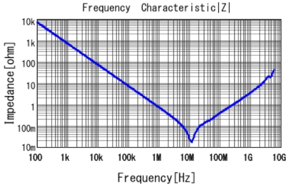
GCM31MR72A224KA37 |Z| DC0V, 25degC
