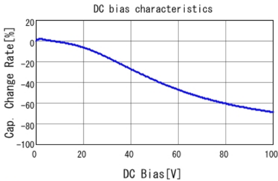
GCM31MR72A224KA37 C-DC bias capchange, 25.0degC, AC1.
