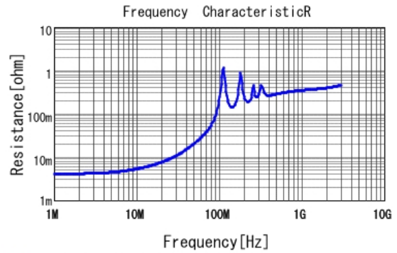
■ GCM32D7U2J103JX01 R DC0V, 25degC
