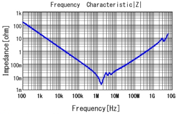
GCM32EC71H106KA03 |Z| DC0V, 25degC
