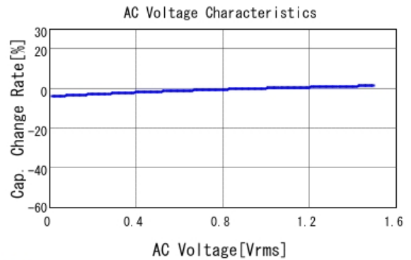
GCM32EC71H106KA03 C-AC Voltage capchange, DC0V, 25.0d
