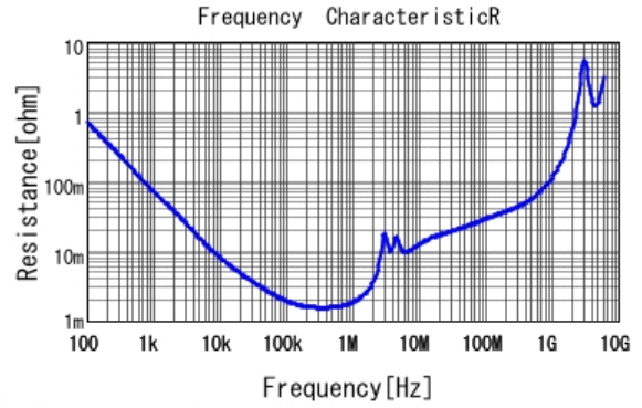
GCM32EC71H106KA03 R DC0V, 25degC
