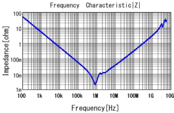
■ GCM32ER70J476ME19 |Z| DCOV, 25degC
