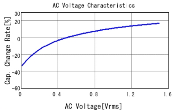
■ GCM32ER70J476ME19 C-AC Voltage capchange, DCOV, 25.0d
