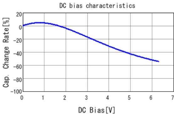
■ GCM32ER70J476ME19 C-DC bias capchange, 25.0degC, AC0.
