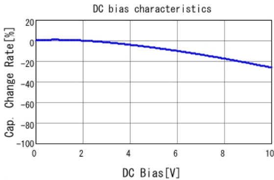
GCM32ER71A226ME12 C-DC bias capchange, 25.0degC, AC0.
