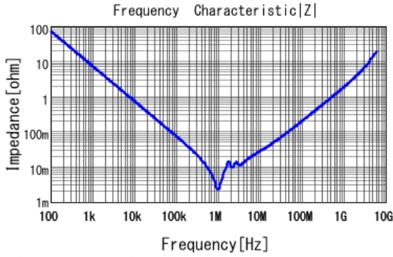
GCM32ER71A226ME12 |Z| DCOV, 25degC
