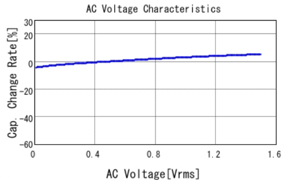
GCM32ER71A226ME12 C-AC Voltage capchange, DCOV, 25.0d
