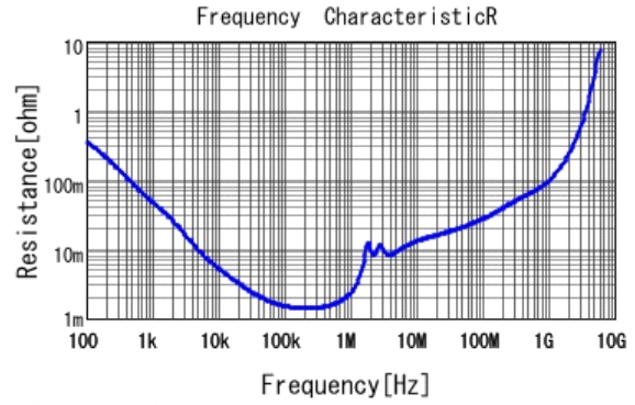
GCM32ER71A226ME12 R DCOV, 25degC
