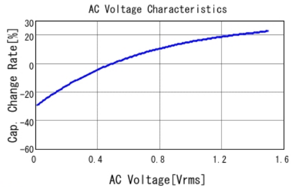
■ GCM32ER71C226ME19 C-AC Voltage capchange, DCOV, 25.0d
