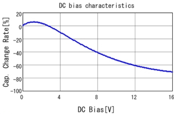
■ GCM32ER71C226ME19 C-DC bias capchange, 25.0degC, AC0.
