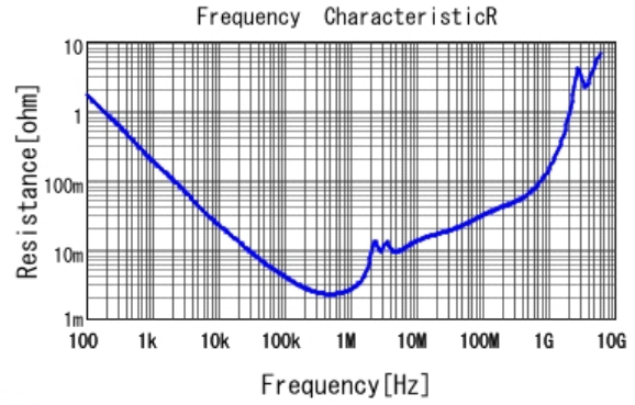
■ GCM32ER71C226ME19 R DCOV, 25degC
