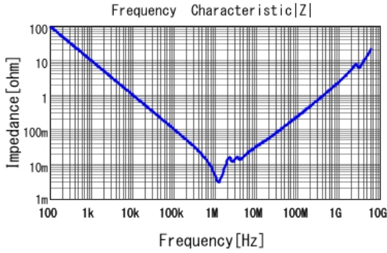
■ GCM32ER71C226ME19 |Z| DCOV, 25degC
