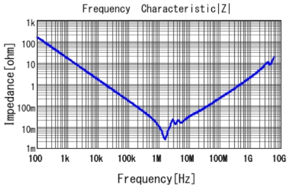
■ GCM32ER71E106KA57 |Z| DC0V, 25degC
