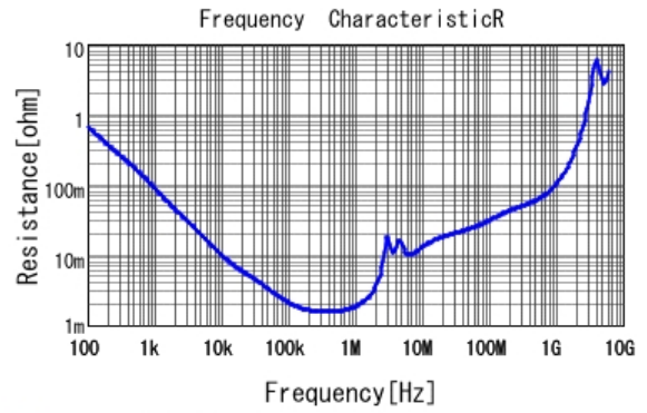
■ GCM32ER71E106KA57 R DC0V, 25degC
