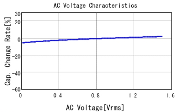
■ GCM32ER71E106KA57 C-AC Voltage capchange, DC0V, 25.0d
