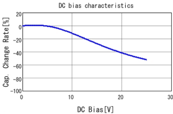
■ GCM32ER71E106KA57 C-DC bias capchange, 25.0degC, AC1.
