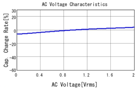
■ GCM32ER71H475KA55 C-AC Voltage capchange, DC0V, 25.0d
