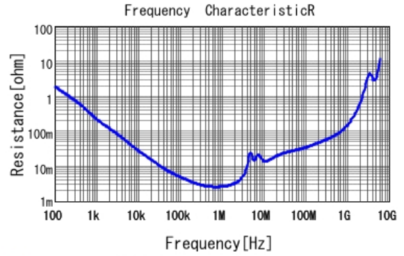
■ GCM32ER71H475KA55 R DC0V, 25degC
