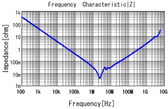
■ GCM32ER71H475KA55 |Z| DC0V, 25degC
