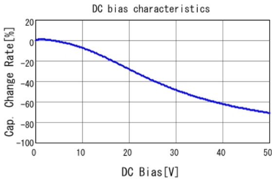
■ GCM32ER71H475KA55 C-DC bias capchange, 25.0degC, AC1.
