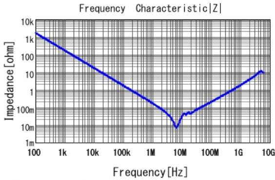
GJ821BR71H105KA12 |Z| DC0V, 25degC
