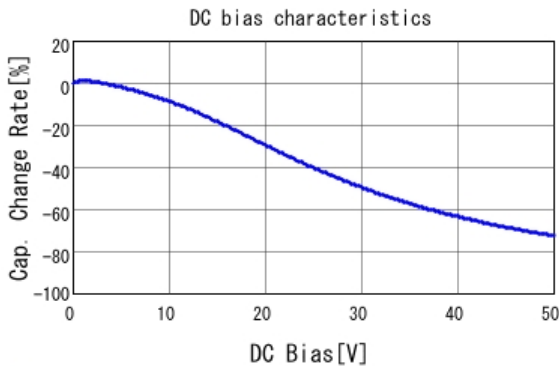
GJ821BR71H105KA12 C-DC bias capchange, 25.0degC, AC1.
