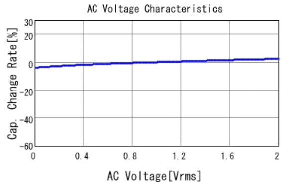
GJ821BR71H105KA12 C-AC Voltage capchange, DC0V, 25.0d
