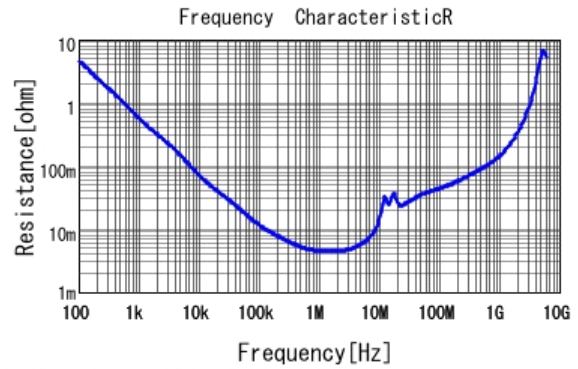
GJ821BR71H105KA12 R DC0V, 25degC
