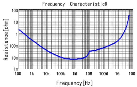
■ GJ831CC81E105KA01 R DCOV, 25degC
