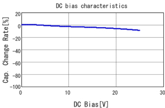
■ GJ831CC81E105KA01 C-DC bias capchange, 25.0degC, AC1.
