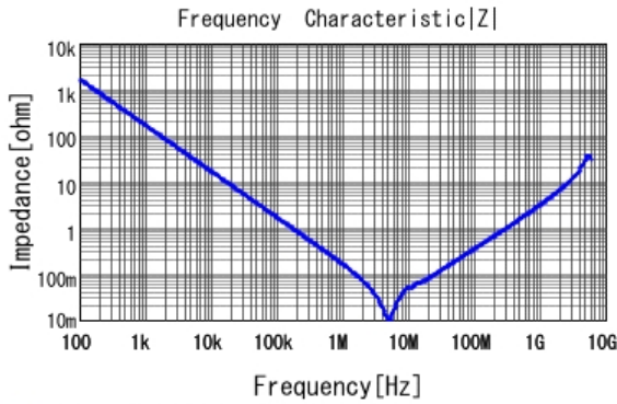
■ GJ831CC81E105KA01 |Z| DCOV, 25degC
