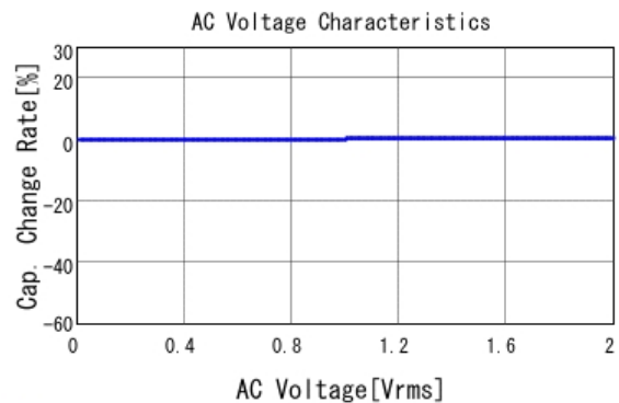
■ GJ831CC81E105KA01 C-AC Voltage capchange, DCOV, 25.0d
