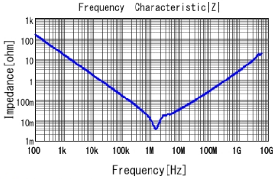
■ GJ831CR61E106KE83 |Z| DC0V, 25degC
