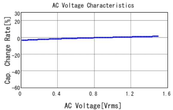
■ GJ831CR61E106KE83 C-AC Voltage capchange, DC0V, 25.0d
