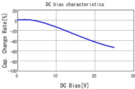
■ GJ831CR61E106KE83 C-DC bias capchange, 25.0degC, AC1.
