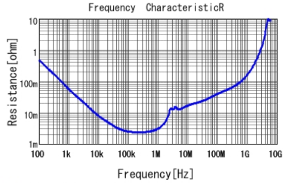
■ GJ831CR61E106KE83 R DC0V, 25degC
