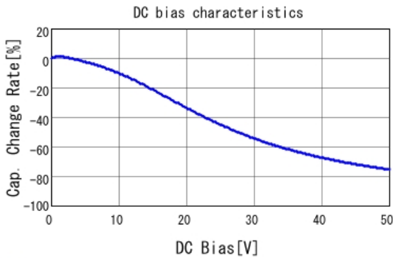
■ GJ831CR71H475KA12 C-DC bias capchange, 25.0degC, AC1.
