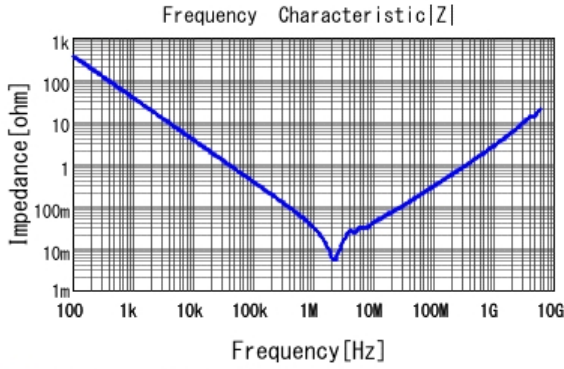
■ GJ831CR71H475KA12 |Z| DC0V, 25degC
