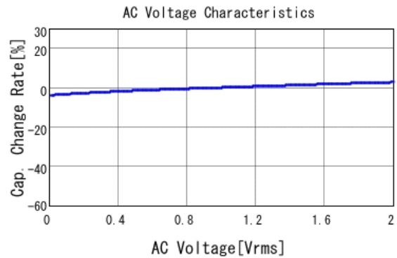
■ GJ831CR71H475KA12 C-AC Voltage capchange, DC0V, 25.0d
