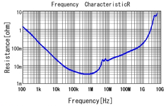
■ GJ831CR71H475KA12 R DC0V, 25degC
