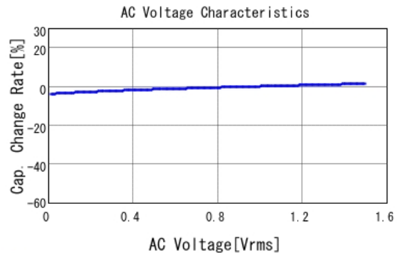
■ GJ832ER7YA106KA12 C-AC Voltage capchange, DCOV, 25.0d
