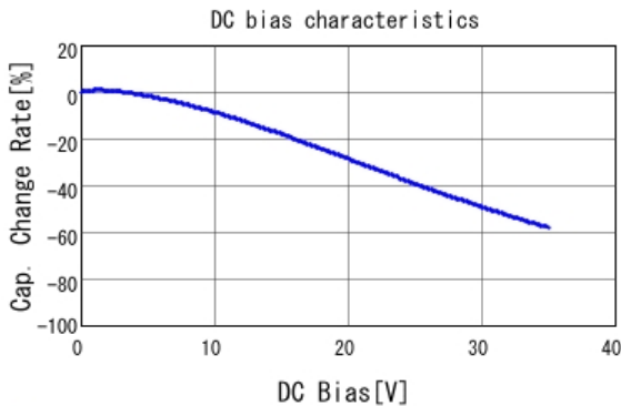
■ GJ832ER7YA106KA12 C-DC bias capchange, 25.0degC, AC1.
