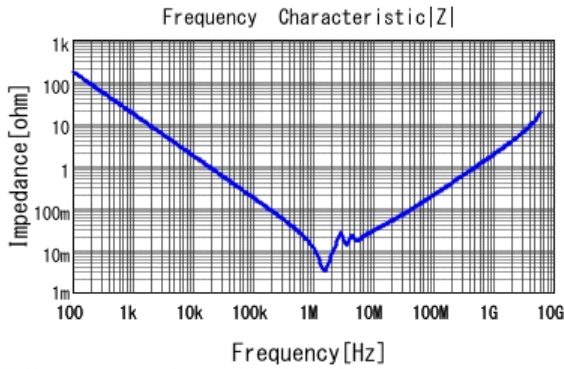
■ GJ832ER7YA106KA12 |Z| DCOV, 25degC
