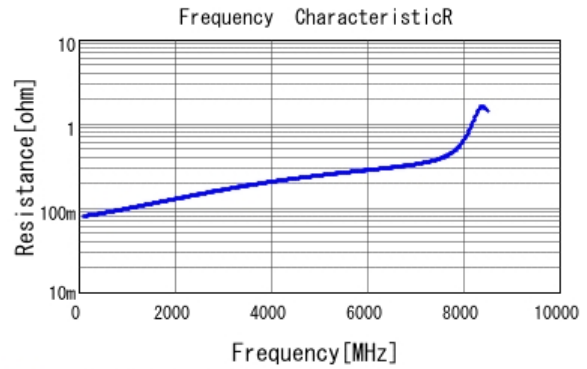
■ GJM0335C1E100GB01 R DC0V, 25degC
