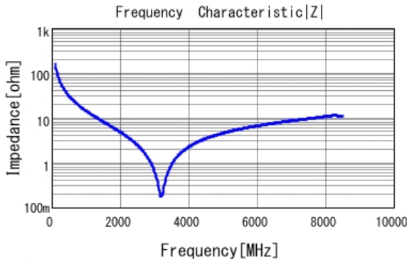
■ GJM0335C1E100GB01 |Z| DC0V, 25degC
