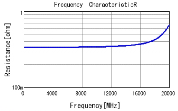
■ GJM0335C1E1R0BB01 R DC0V, 25degC
