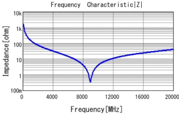
■ GJM0335C1E1R0BB01 |Z| DC0V, 25degC
