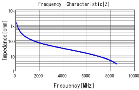
■ GJM0335C1E1R1BB01 |Z| DC0V, 25degC
