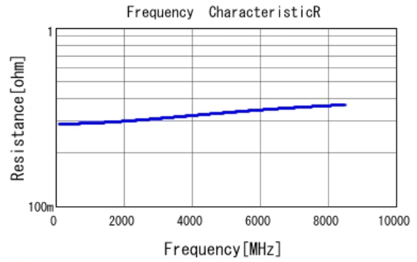
■ GJM0335C1E1R1BB01 R DC0V, 25degC
