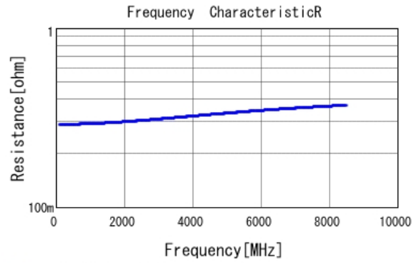
■ GJM0335C1E1R2WB01 R DCOV, 25degC
