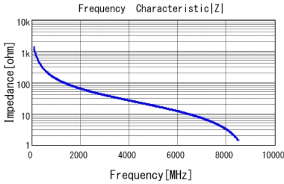
■ GJM0335C1E1R2WB01 |Z| DCOV, 25degC
