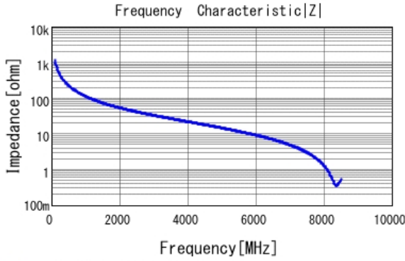
■ GJM0335C1E1R4BB01 |Z| DC0V, 25degC
