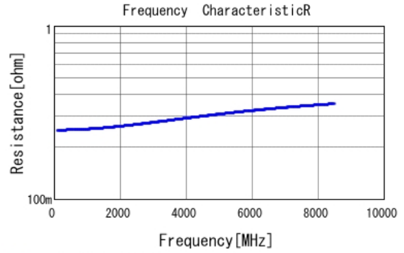
■ GJM0335C1E1R4BB01 R DC0V, 25degC
