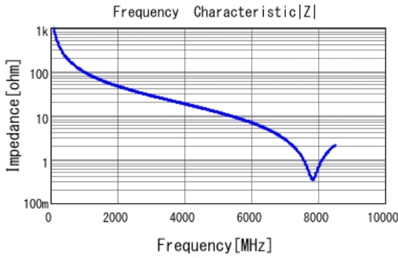
■ GJM0335C1E1R6BB01 |Z| DC0V, 25degC
