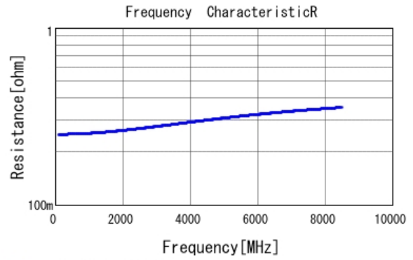
■ GJM0335C1E1R6BB01 R DC0V, 25degC
