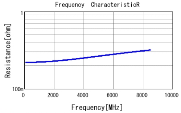
■ GJM0335C1E1R8BB01 R DC0V, 25degC
