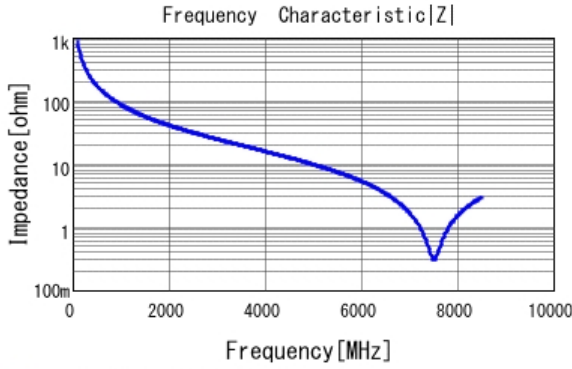
■ GJM0335C1E1R8BB01 |Z| DC0V, 25degC
