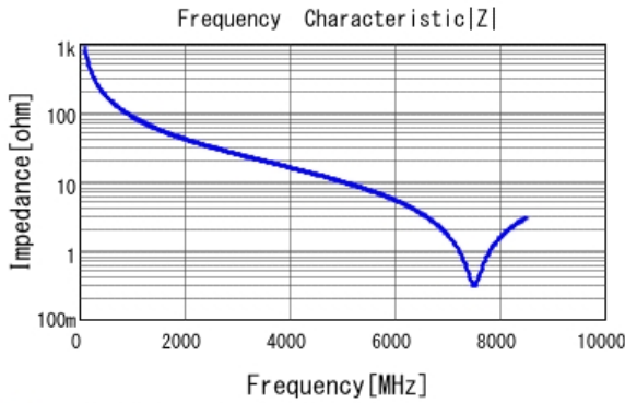
■ GJM0335C1E1R8CB01 |Z| DCOV, 25degC
