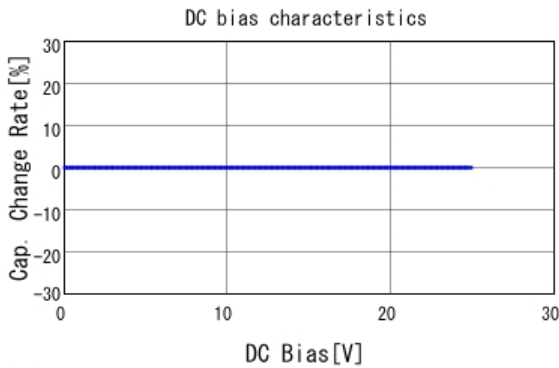
■ GJM0335C1E1R8CB01 C-DC bias capchange, 25.0degC, AC1V
