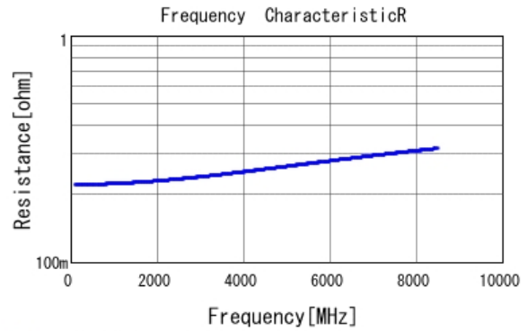
■ GJM0335C1E1R8CB01 R DCOV, 25degC
