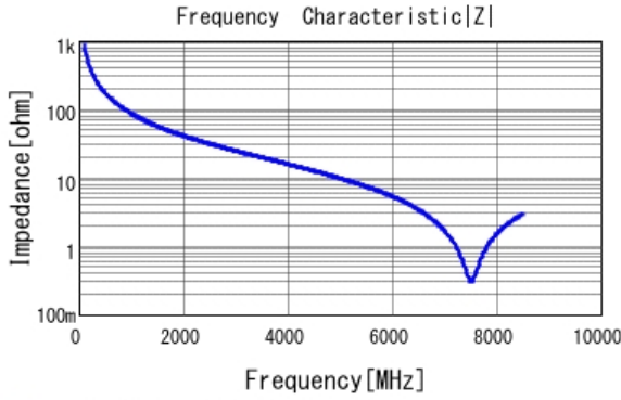
■ GJM0335C1E1R8WB01 |Z| DCOV, 25degC
