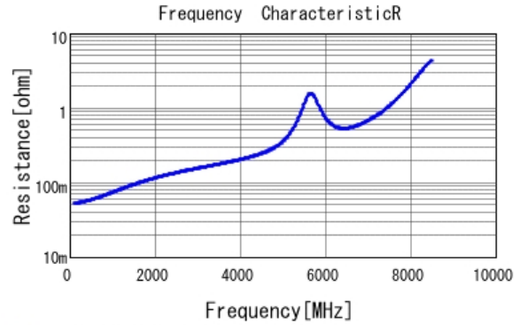
■ GJM0335C1E220JB01 R DC0V, 25degC
