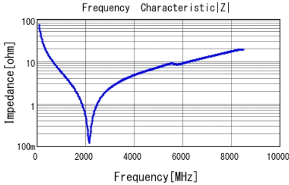
■ GJM0335C1E220JB01 |Z| DC0V, 25degC
