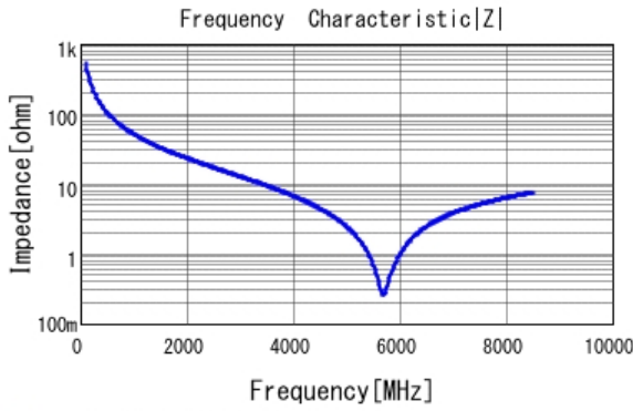
■ GJM0335C1E3R0BB01 |Z| DCOV, 25degC
