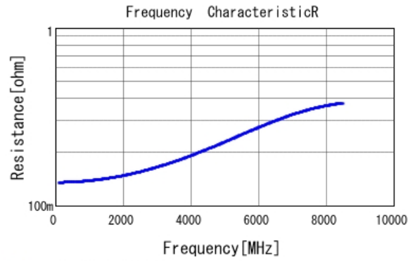
■ GJM0335C1E3R0BB01 R DCOV, 25degC
