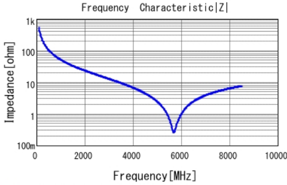
■ GJM0335C1E3R0WB01 |Z| DCOV, 25degC
