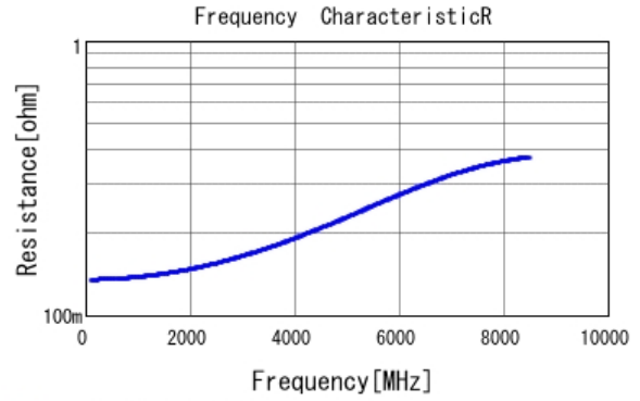
■ GJM0335C1E3R0WB01 R DCOV, 25degC
