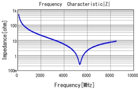
■ GJM0335C1E3R3BB01 |Z| DCOV, 25degC
