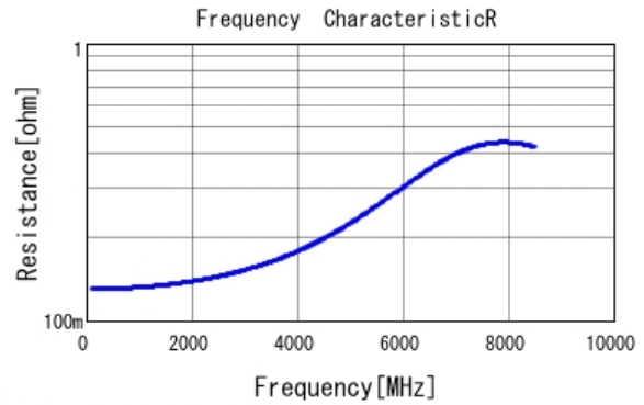
■ GJM0335C1E3R3BB01 R DCOV, 25degC
