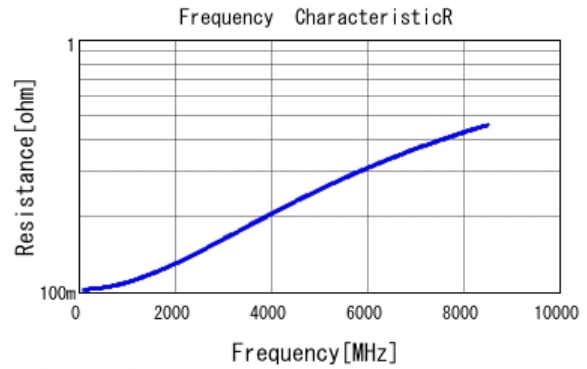
■ GJM0335C1E4R3BB01 R DC0V, 25degC
