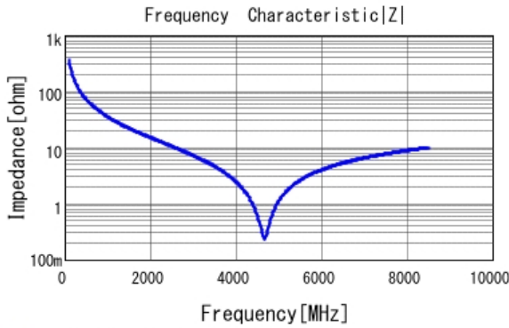
■ GJM0335C1E4R3BB01 |Z| DC0V, 25degC
