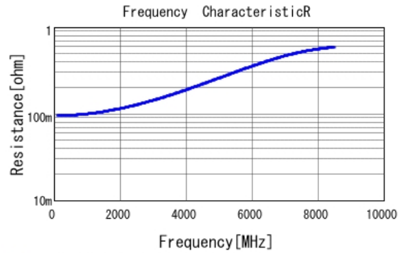
■ GJM0335C1E5R0BB01 R DCOV, 25degC
