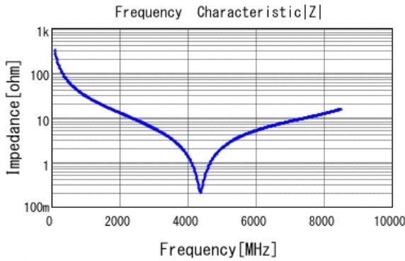
■ GJM0335C1E5R0BB01 |Z| DCOV, 25degC
